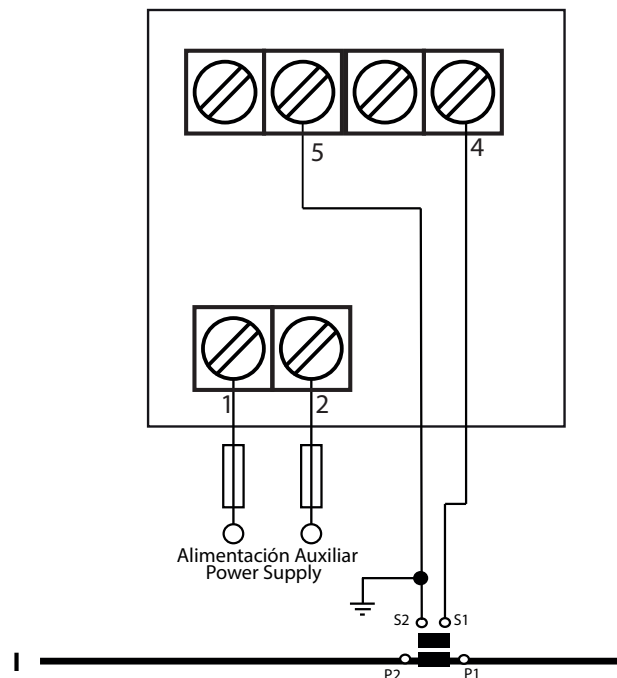
Figure 4: Current measurement DCB-48 Aac.
