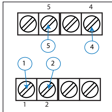
Figure 3:Terminals of the DCB-48 Aac.
