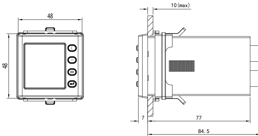
Figure 13: Dimensions of the DCB-48 Aac.
