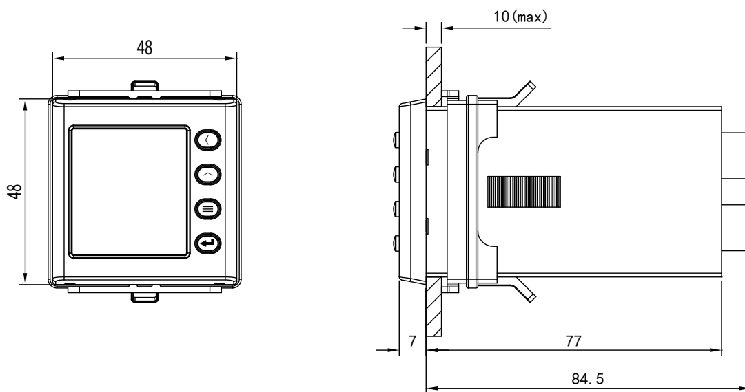
Figure 13: Dimensions of the DCB-48 Adc.
