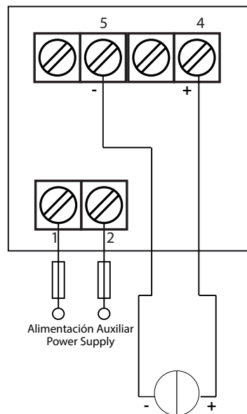
Figure 4: Current measurement DCB-48 Adc.
