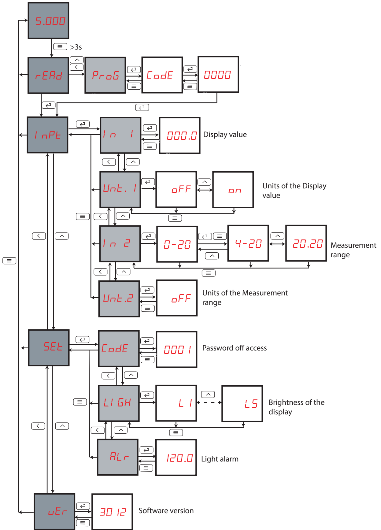
Figure 14: Configuration menu DCB-48 mAdc
