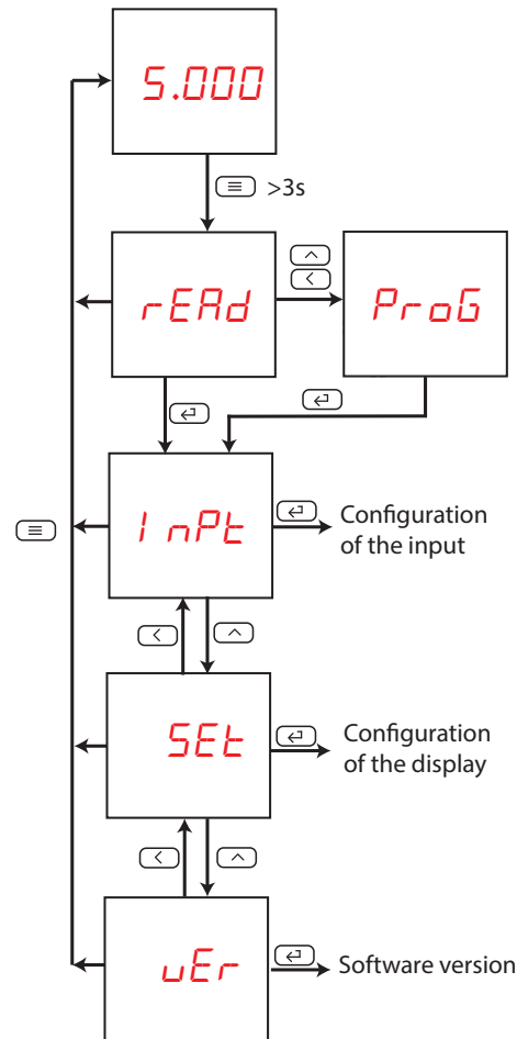
Figure 6: Configuration menu of the DCB-48 Adc.
