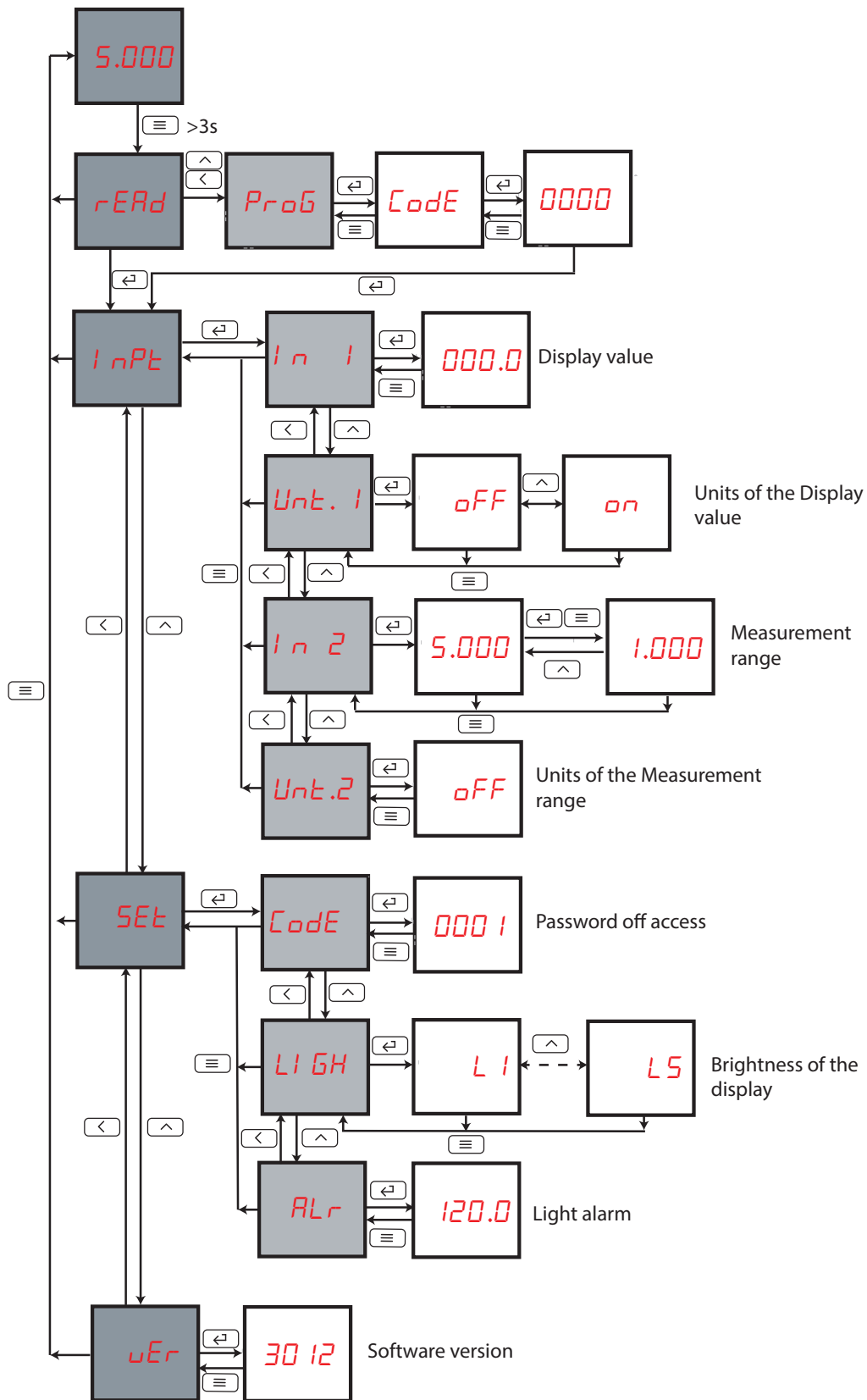
Figure 15: Configuration menu DCB-48 Adc
