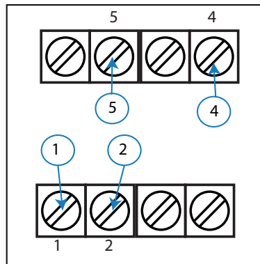
Figure 3:Terminals of the DCB-48 Adc.
