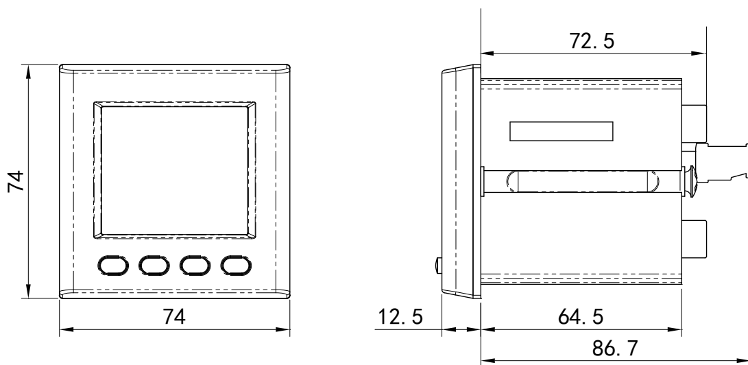
Figure 16: Dimensions of the DCB-72 Vac.
