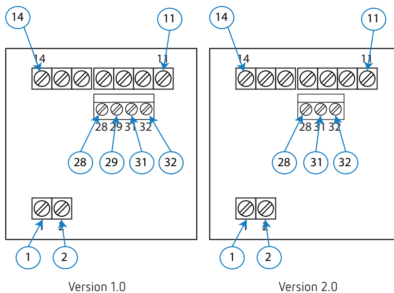
Figure 3:Terminals of the DCB-72 Vac.
