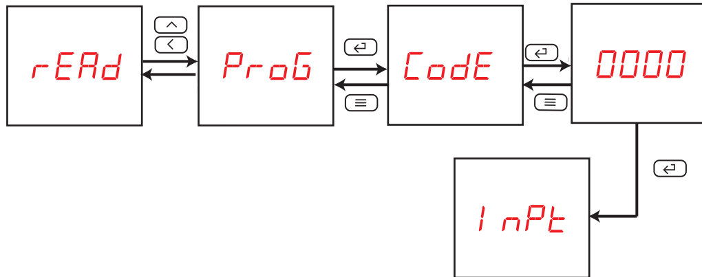
Figure 7: Access the configuration menu in the programming mode.
