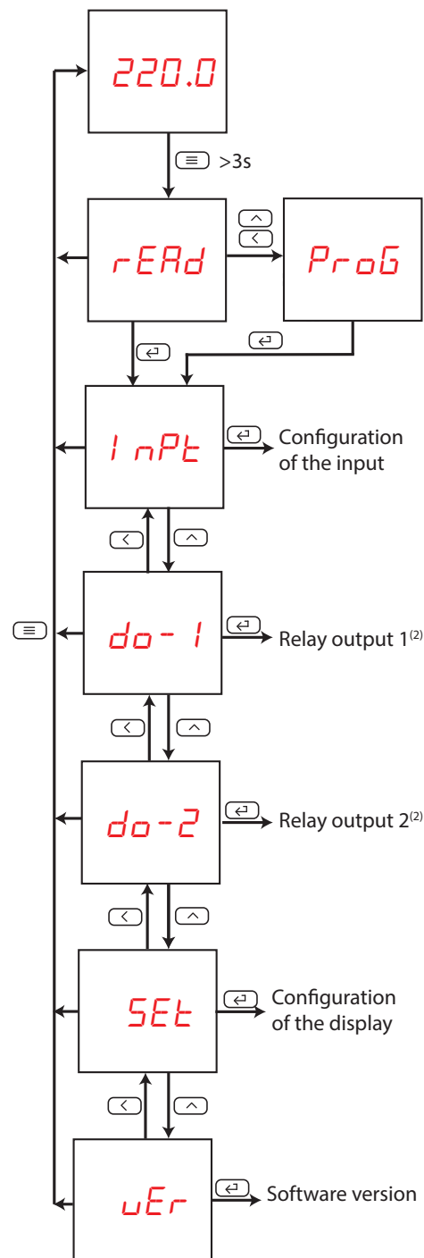
Figure 6: Configuration menu of the DCB-72 Vac.
