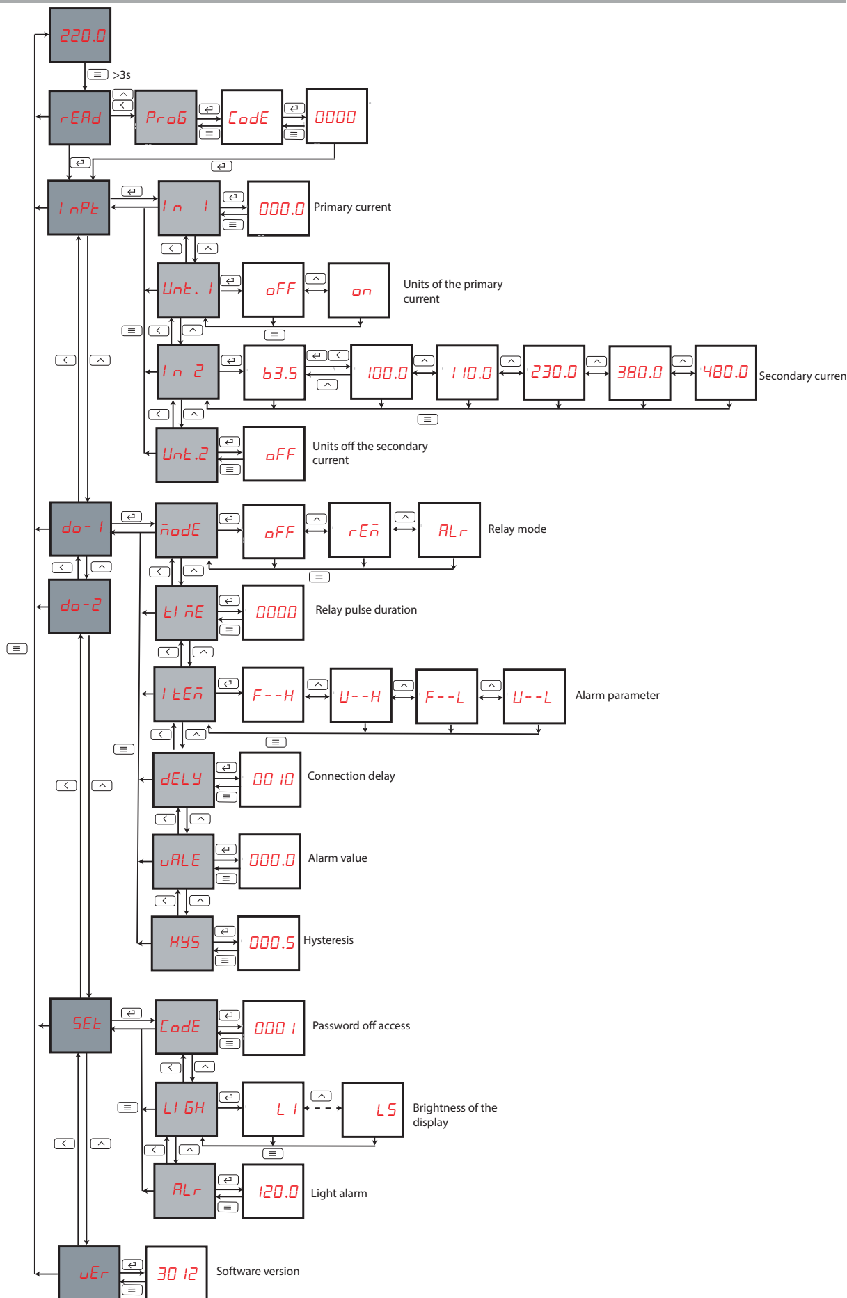
Figure 18: Configuration menu DCB-72 Vac (with relays)
