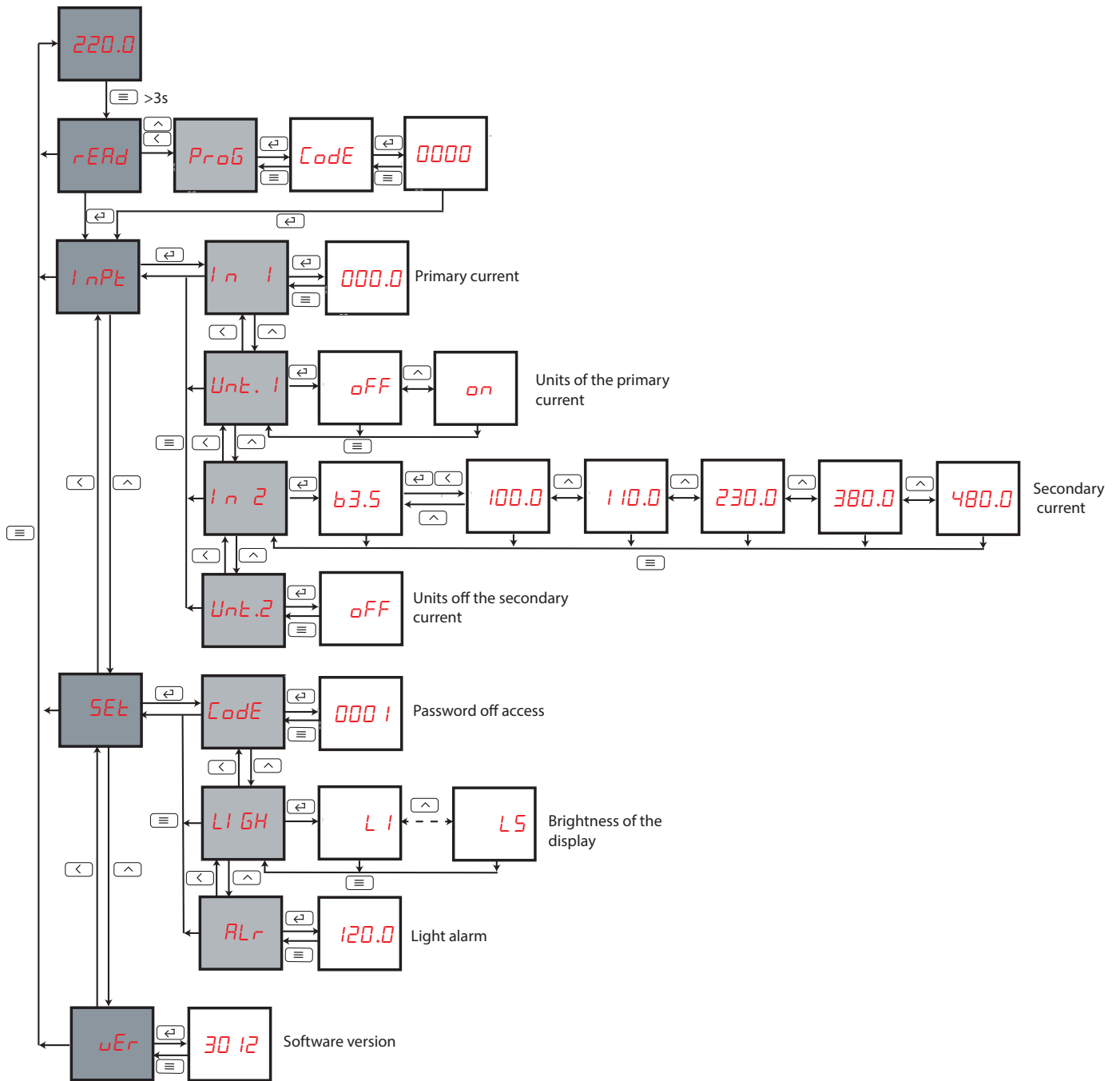
Figure 17: Configuration menu DCB-72 Vac
