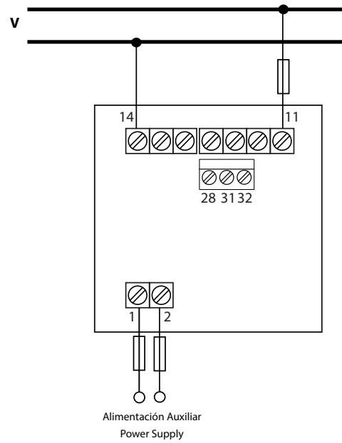
Figure 4: Voltage measurement DCB-72 Vac.
