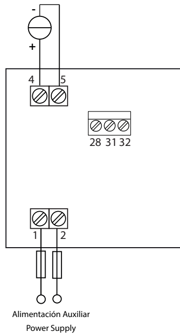
Figure 4: Current measurement DCB-72 Adc.
