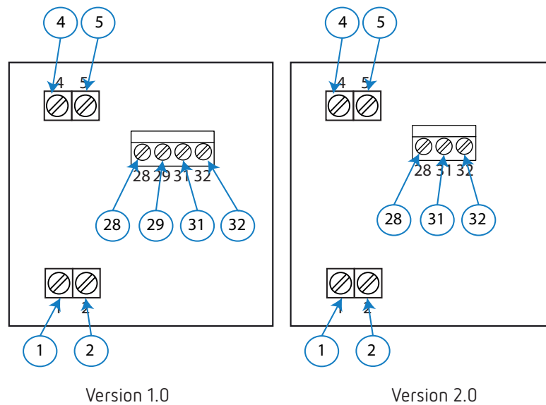
Figure 3:Terminals of the DCB-72 Adc.
