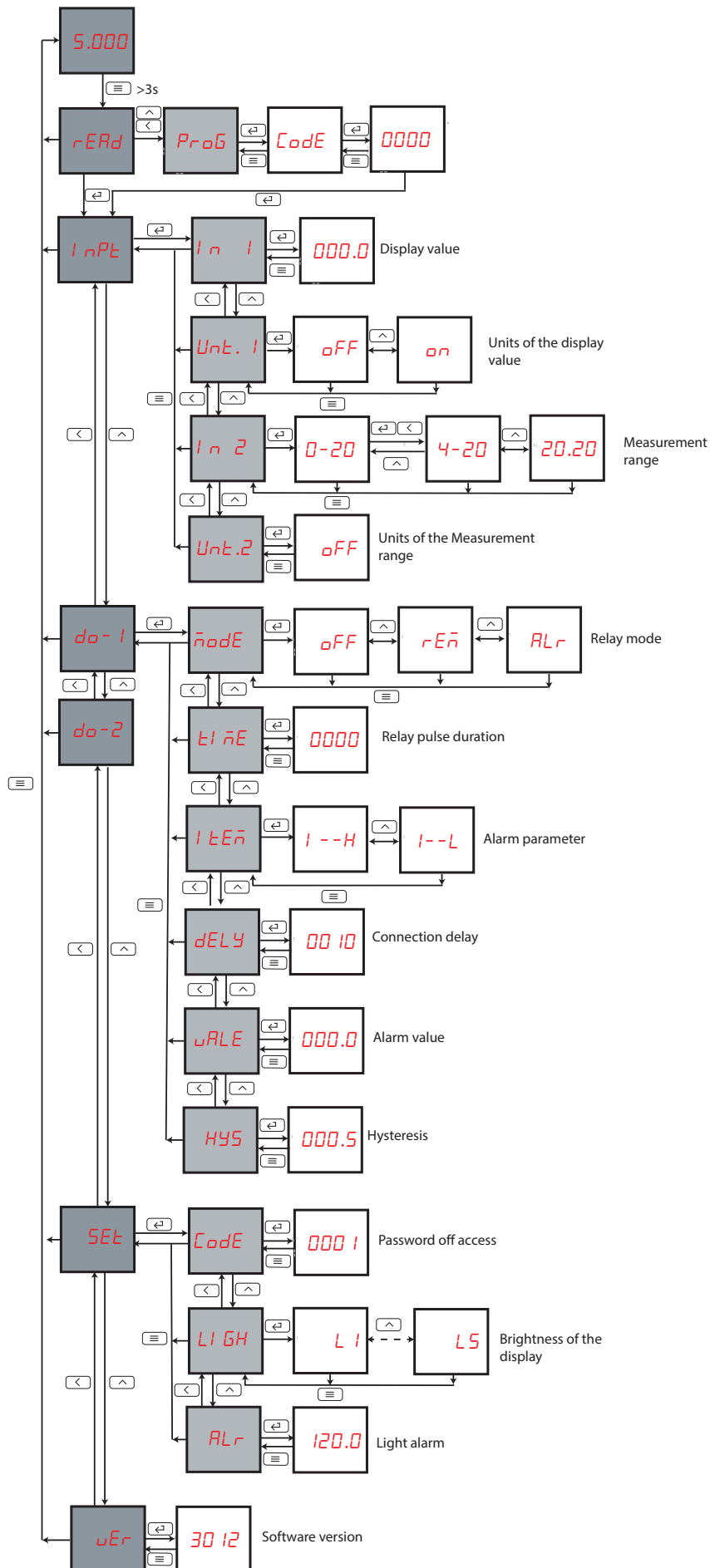
Figure 18: Configuration menu DCB-72 mAdc (with relays)
