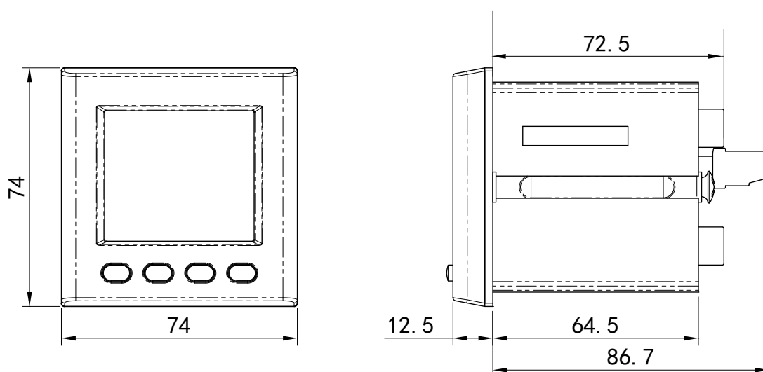
Figure 16: Dimensions of the DCB-72 Adc.
