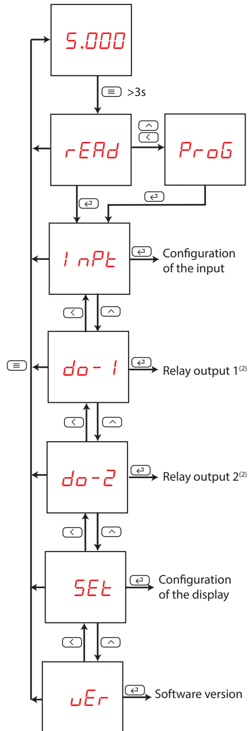
Figure 6: Configuration menu of the DCB-72 Adc.
