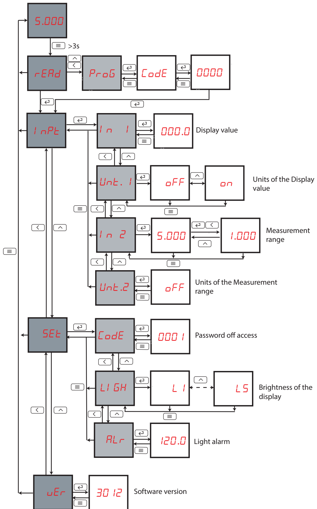
Figure 19: Configuration menu DCB-72 Adc
