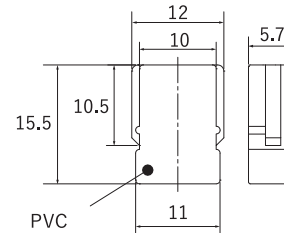
PVC mounting bracket
